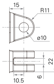
6 = Aluminum casting, clevis U, slot 6, depth 10.5, hole 10, one piece casting with gear box
