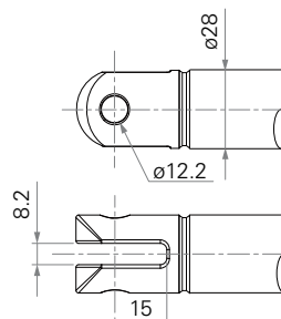
5 = Aluminum casting, clevis U, slot 8.2, depth 15, hole 12.2 (IP: IP66D, IP69K)
