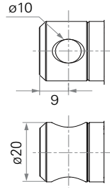
3 = Aluminum casting, no slot, hole 10
