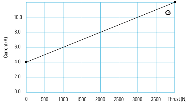
Current vs. Thrust
