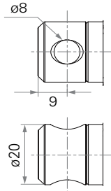
2 = Aluminum casting, no slot, hole 8
