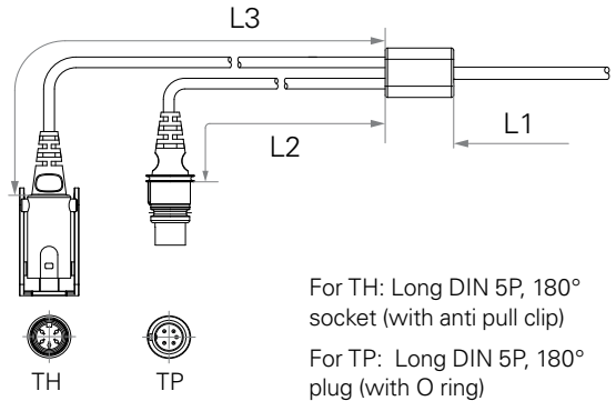
C = Y cable, for direct cut system
