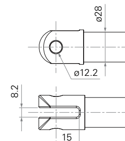
5 = Aluminum casting, clevis U, slot 8.2, depth 15, hole 12.2 (IP: Without, IP54)
