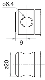
1 = Aluminum casting, no slot, hole 6.4
